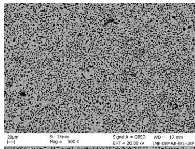
Figure 1 – SEM of porous silicon compact.
